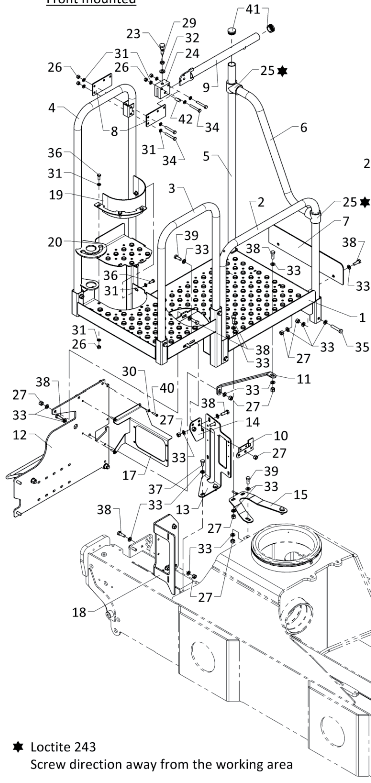
Front mounted
