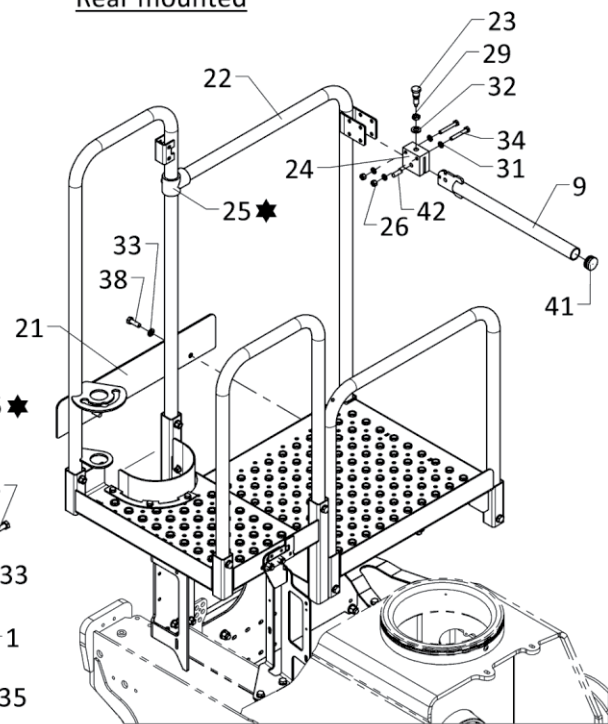
Rear mounted
