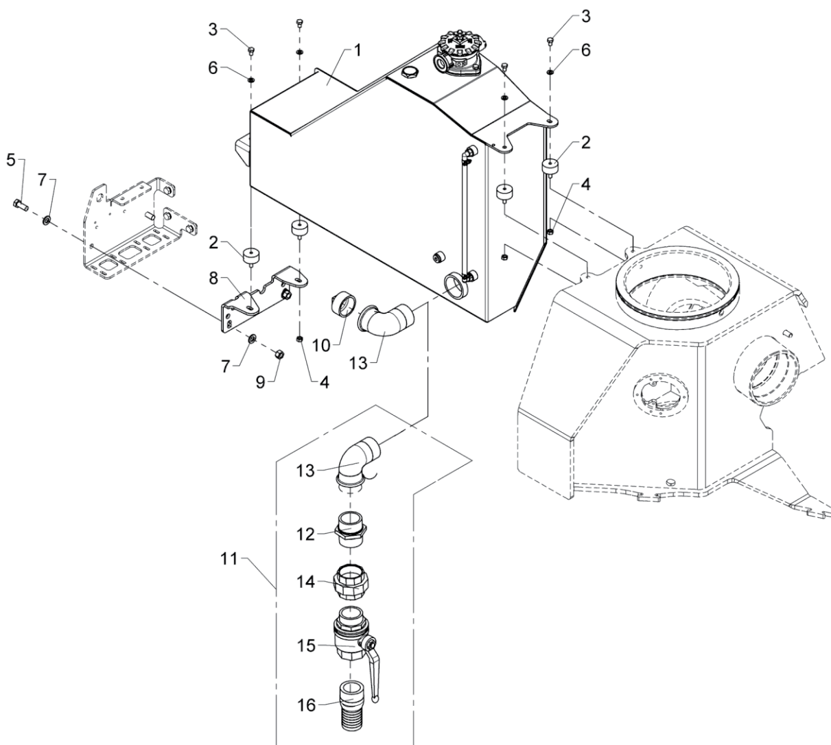
Placement of mounting brackets 6340557 1300K/1730K
