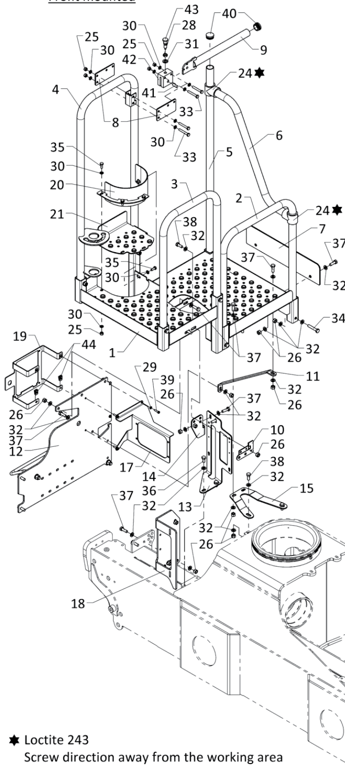
Front mounted
