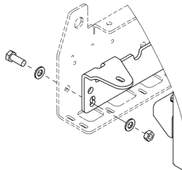
Placement of mounting brackets 6340557 1800K/2430K
