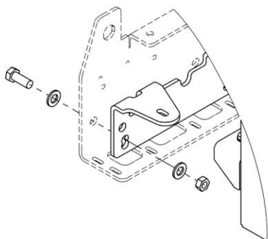
Placement of mounting brackets 6340557 1300K/1730K
