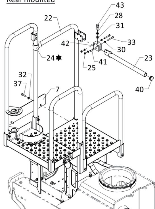
Rear mounted
