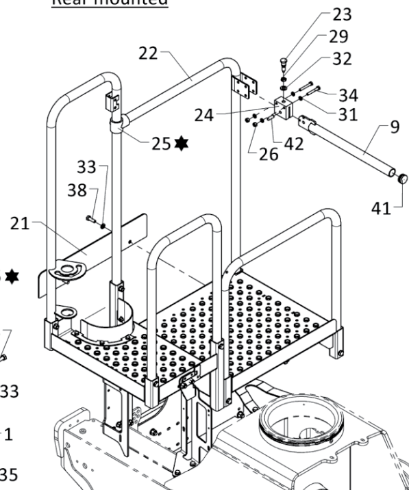
Rear mounted
