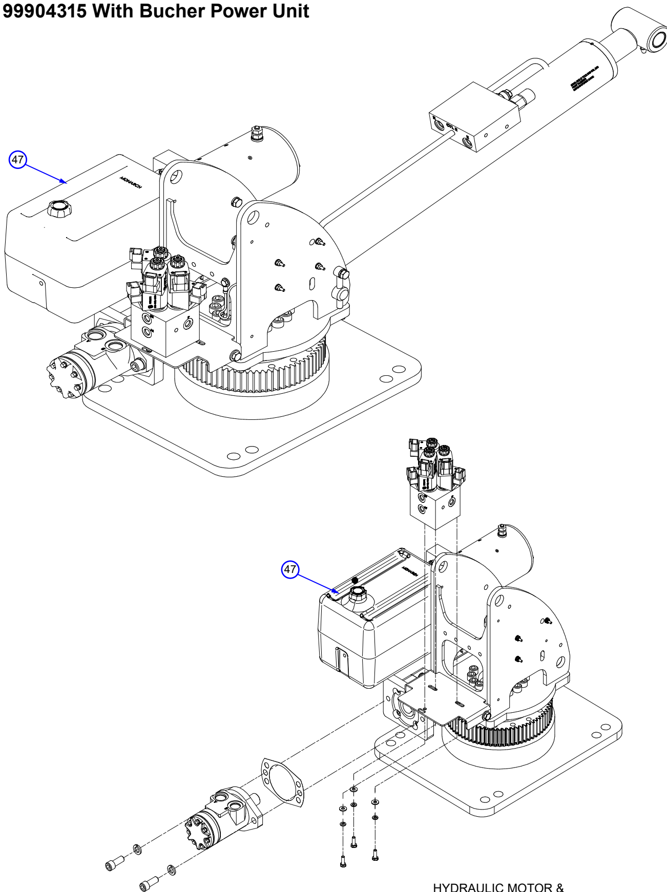
HYDRAULIC MOTOR & VALVE BANK ASSEMBLY
