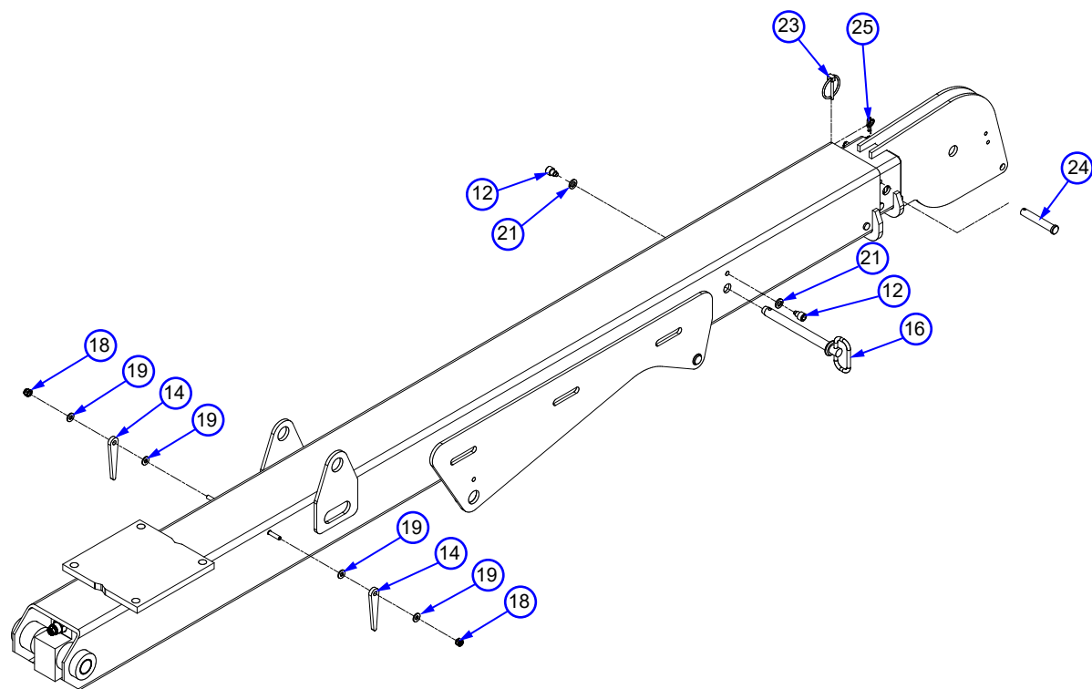
BOOM ASSEMBLY 1 MANUAL EXTENSION
