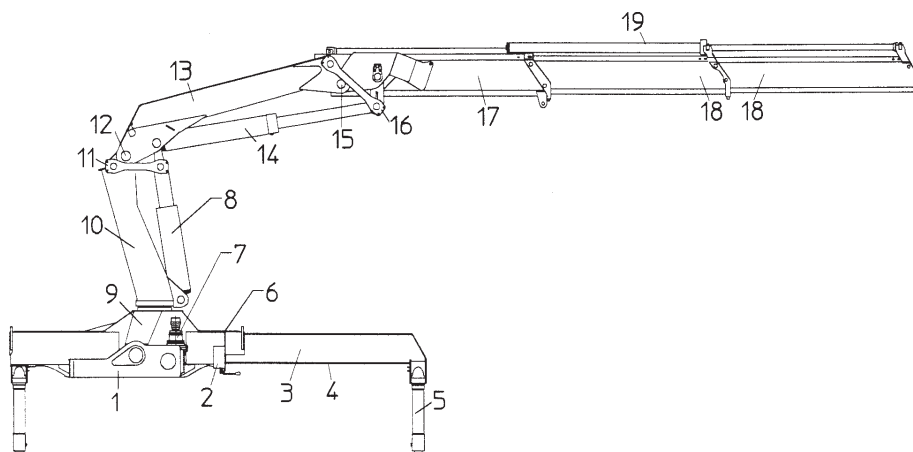
COMPONENT REFERENCE
