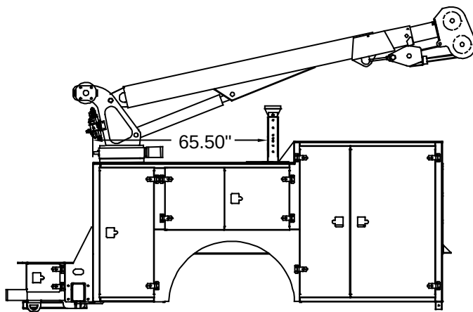
DOMINATOR WITH 3820-5020-6025 CRANE
