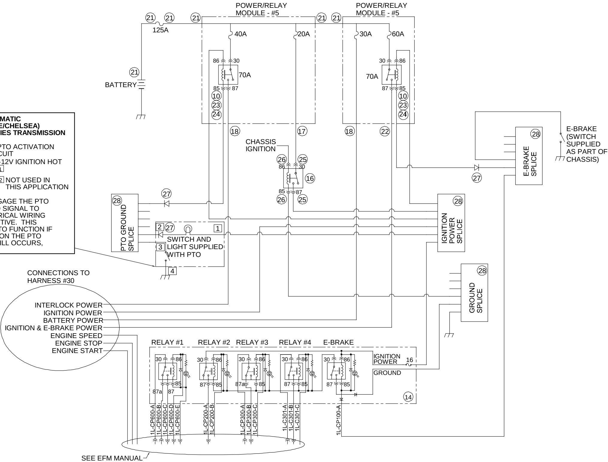
99904034 DRAWING
