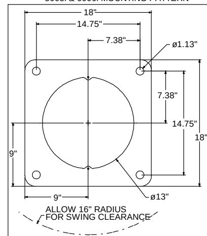
5005i & 6006i MOUNTING PATTERN
