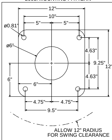
2003i MOUNTING PATTERN
