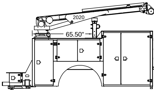
DOMINATOR WITH 2020 CRANE
