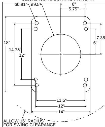
3203i & 4004i MOUNTING PATTERN
