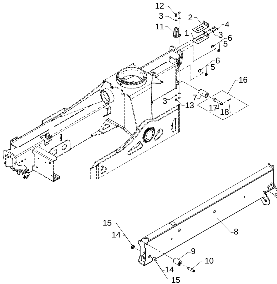
Stabilizer beam, type SH-4600 (53302090A)
