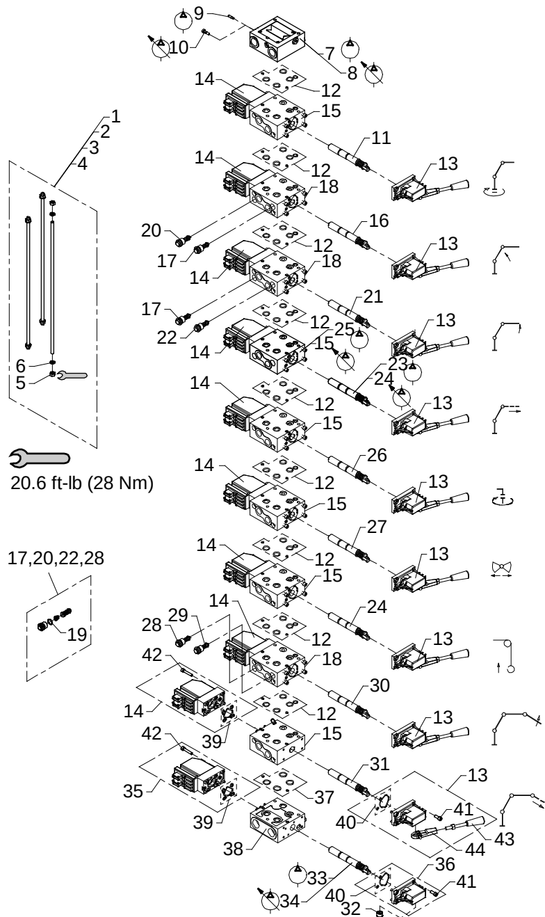
Danfoss control valve PVG32, 4-7 sections (53306490)
