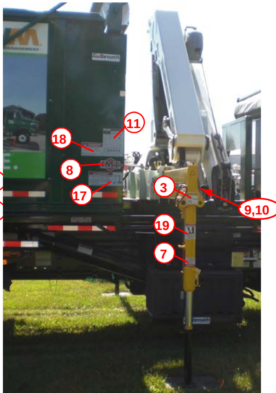
DECALS-PASSENGER SIDE
