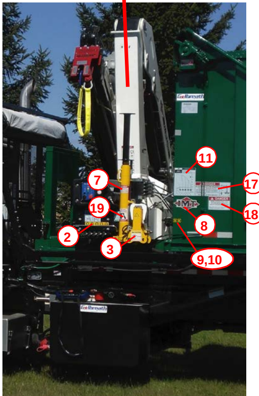
DECALS-DRIVER SIDE
