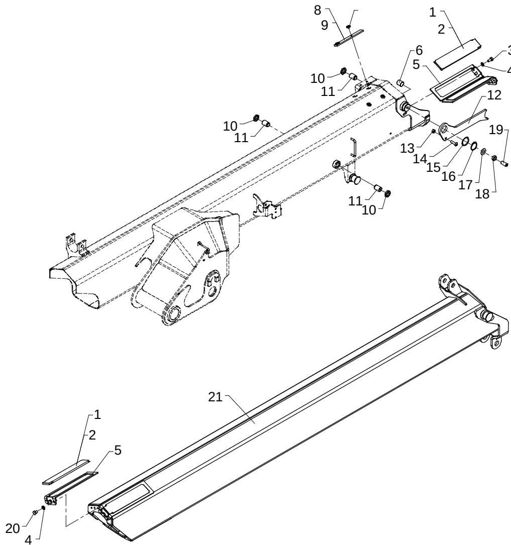
Jib extension K1 incl. fittings (53303105)
