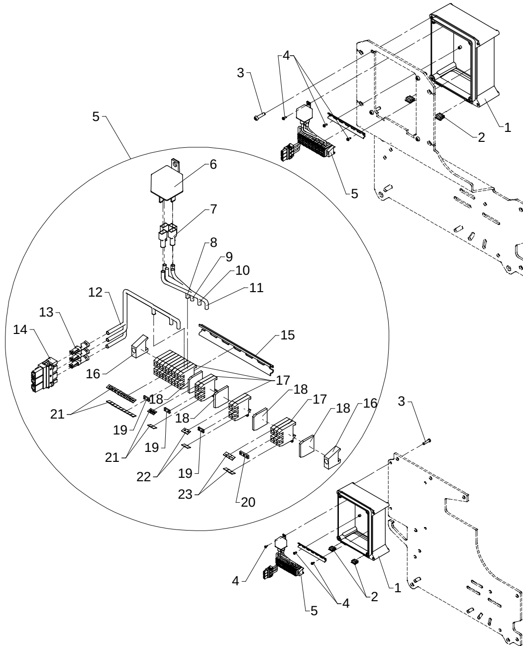
24 V bottom for RCL box with RC (53320050)
