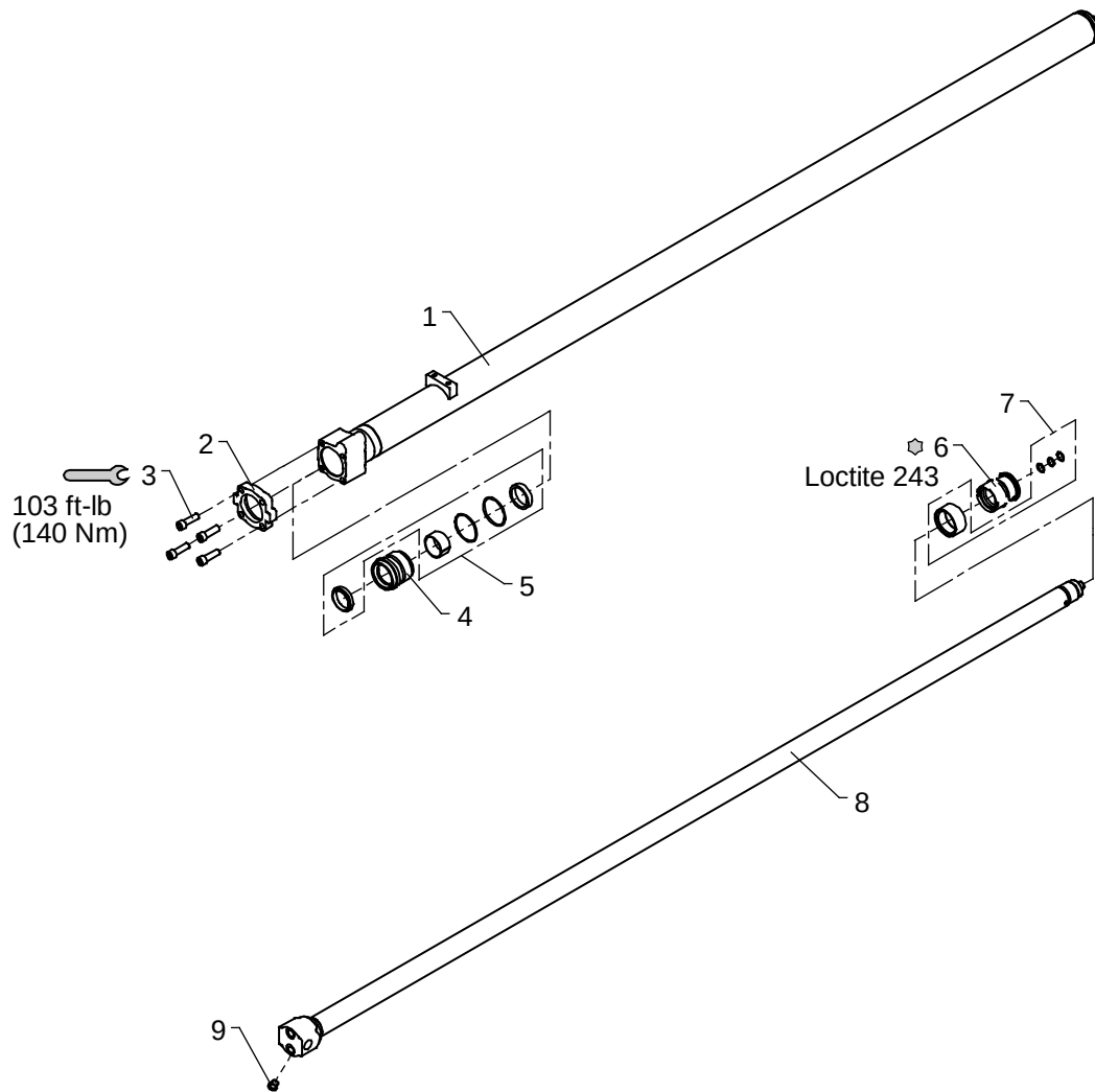
Extension cylinder III (C63/45 x 2100) (53303320)
