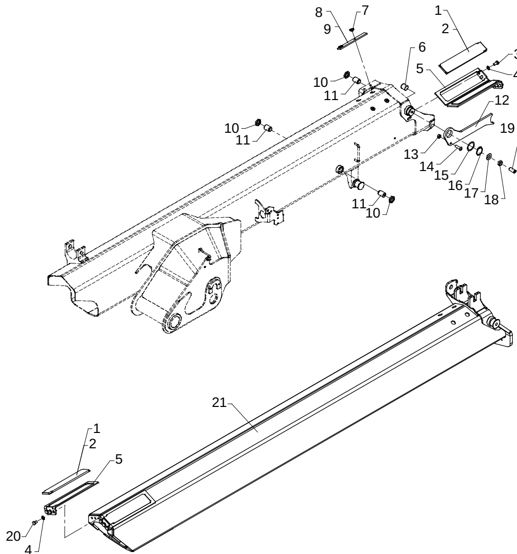
Jib extension I incl. fittings (53303100)
