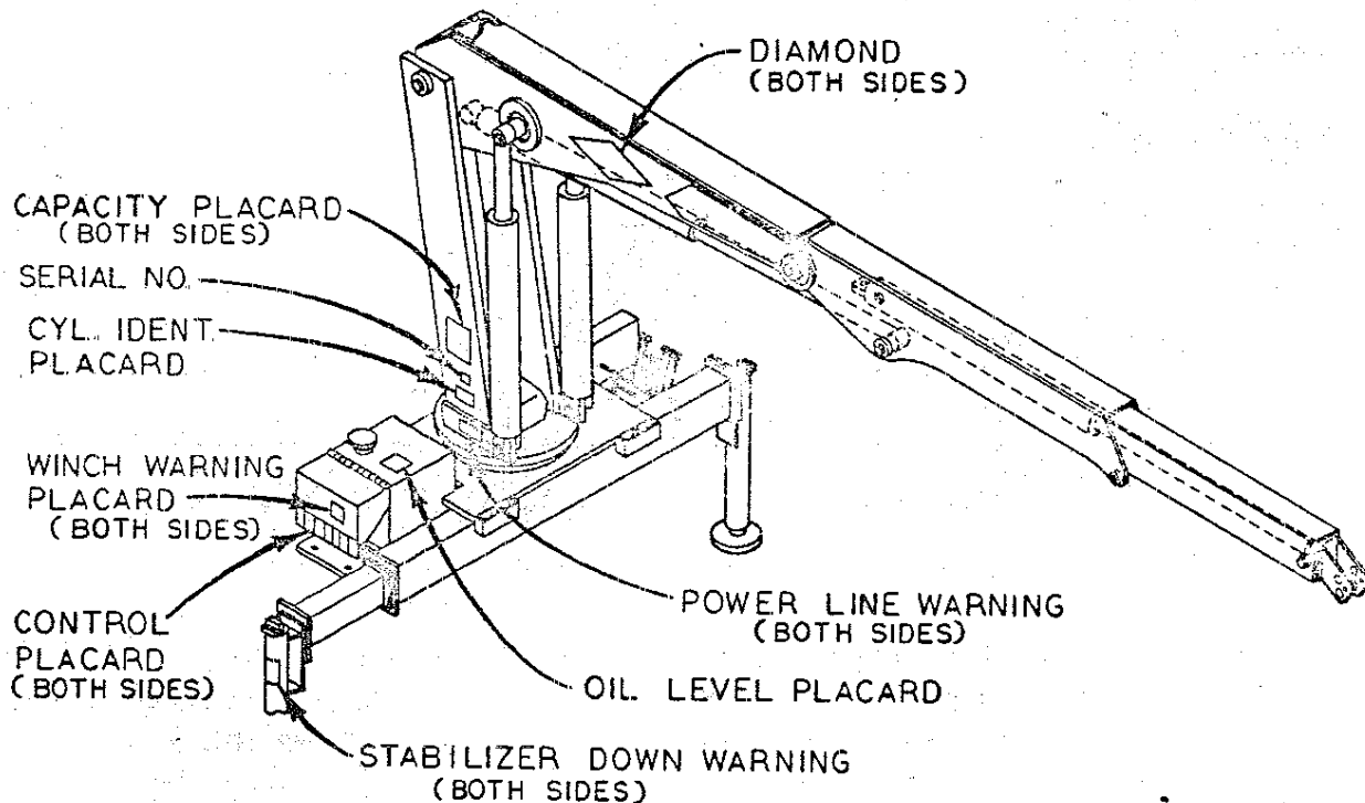
PLACARD PLACEMENT
