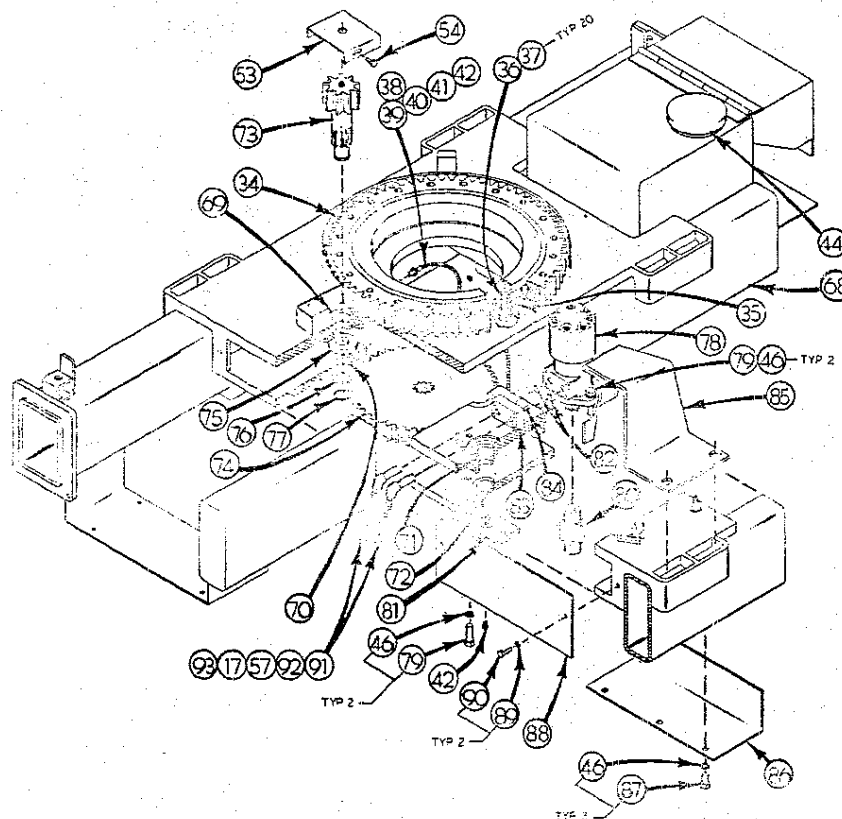
BASE ASSEMBLY WITH GEAR TRAIN ROTATION
