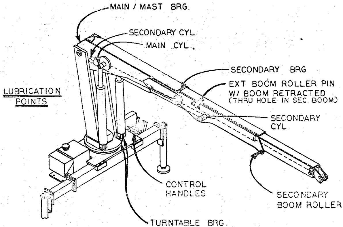
LUBRICATION CHART
