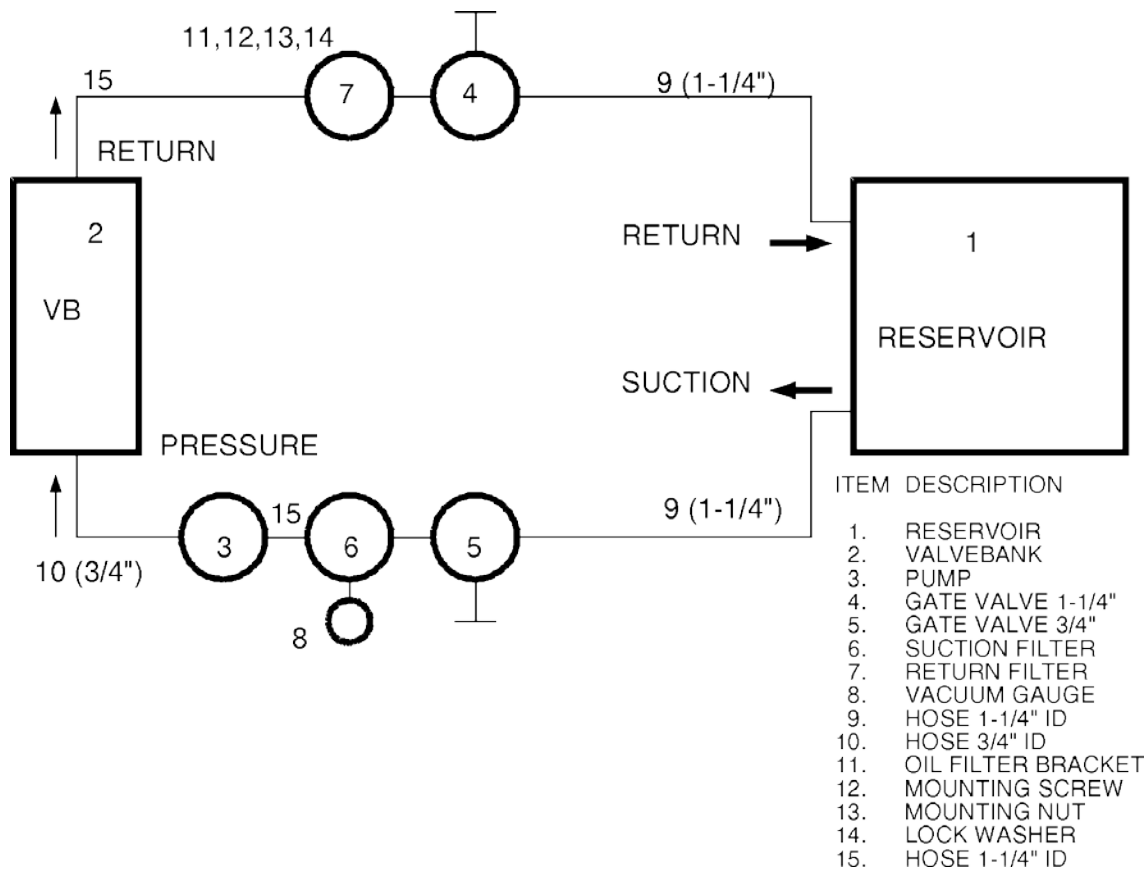
HYDRAULIC INSTALLATION
