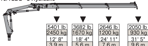
10/72DL - 4 Hydraulic
