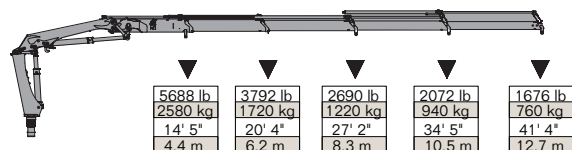
12/86DL - 5 Hydraulic
