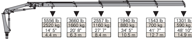
12/86SL - 5 Hydraulic
