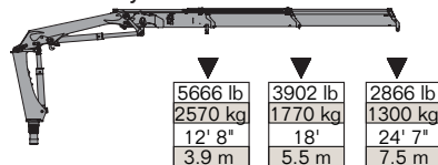
10/72DL - 3 Hydraulic
