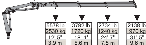
10/72SL - 4 Hydraulic
