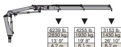
12/86DL - 3 Hydraulic
