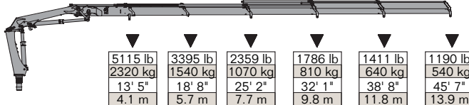
10/72SL - 5 Hydraulic
