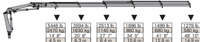
12/86DL - 5 Hydraulic
