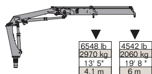
12/86DL - 2 Hydraulic
