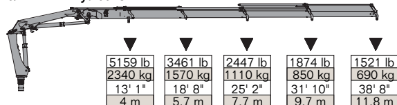
10/72DL - 5 Hydraulic
