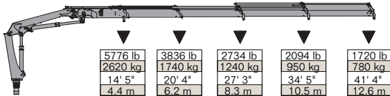
12/86SL - 4 Hydraulic
