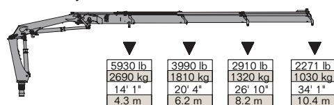
12/86DL - 4 Hydraulic
