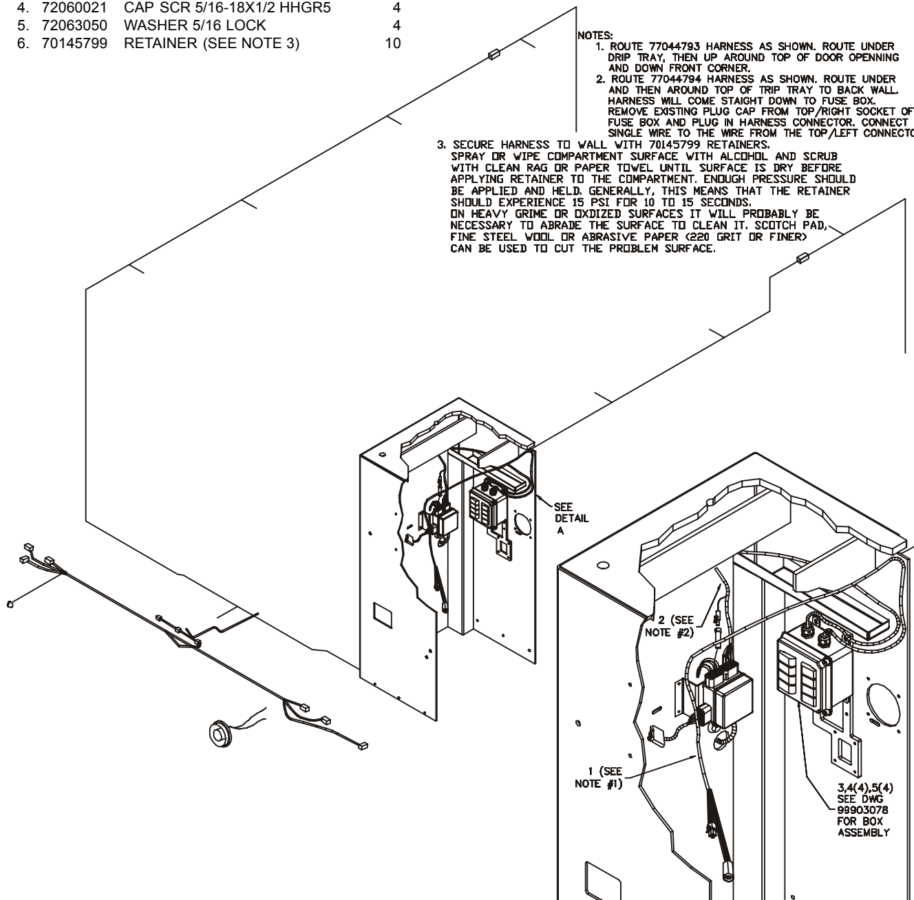
DETAIL A
