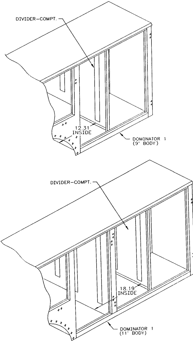
STANDARD BODY SHOWN
