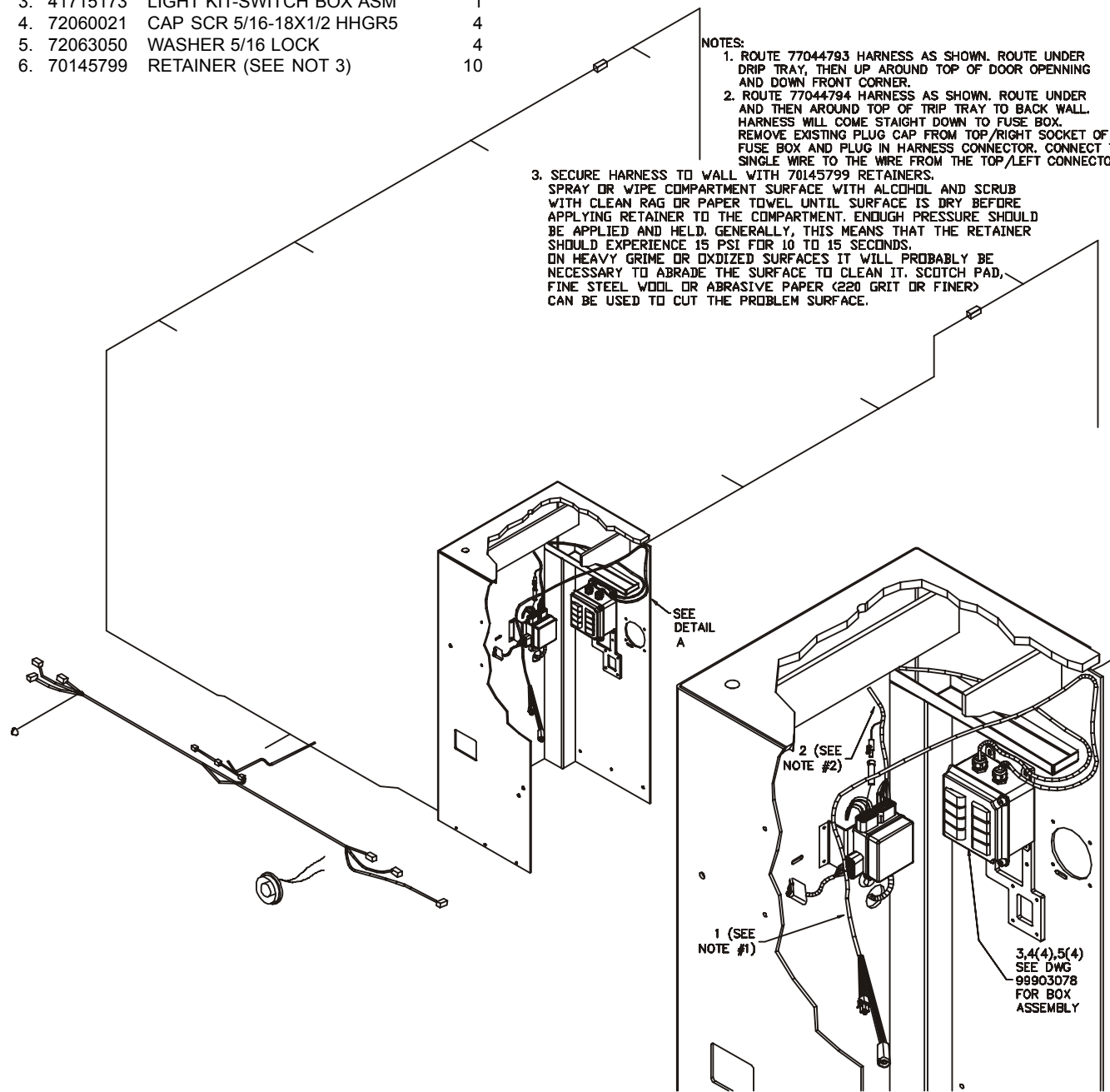
DETAIL A
