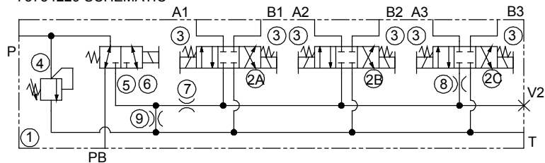
73734229 SCHEMATIC
