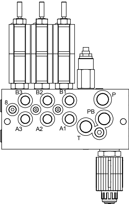
99904403-2 Drawing
