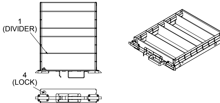
SAMPLE DRAWING - DRAWER WITH 4 DIVIDERS
