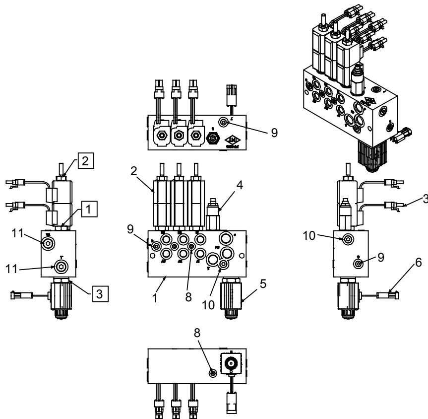
73734229 SCHEMATIC
