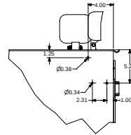
DETAIL B SCALE 1 / 4 DIMS TYPICAL BOTH SIDES STANDARD FRONT BRACKET LOCATION
