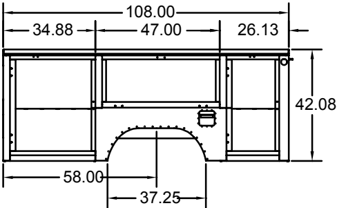
DSS 9' OVERALL DIMENSIONS
