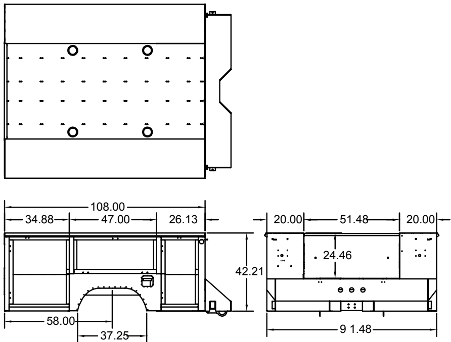
DSC20 9' OVERALL DIMENSIONS
