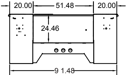
DSS 9' OVERALL DIMENSIONS
