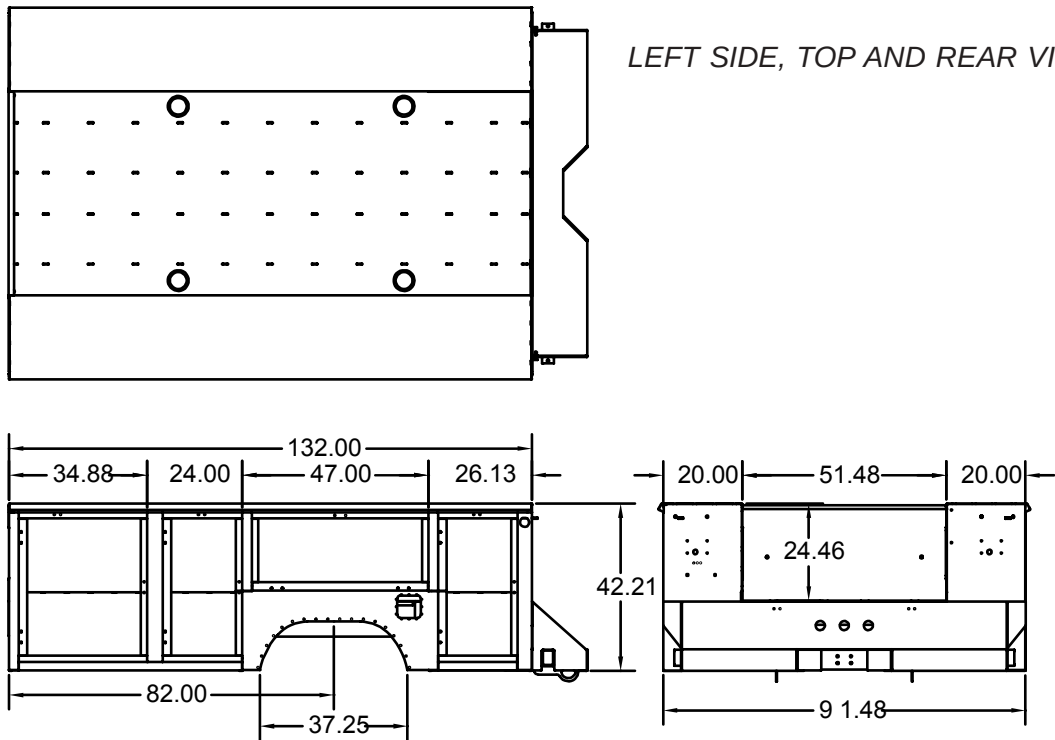
DSC20 11' OVERALL DIMENSIONS
