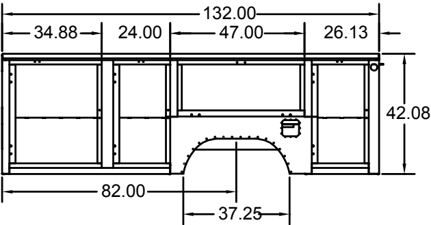
DSS 11' OVERALL DIMENSIONS
