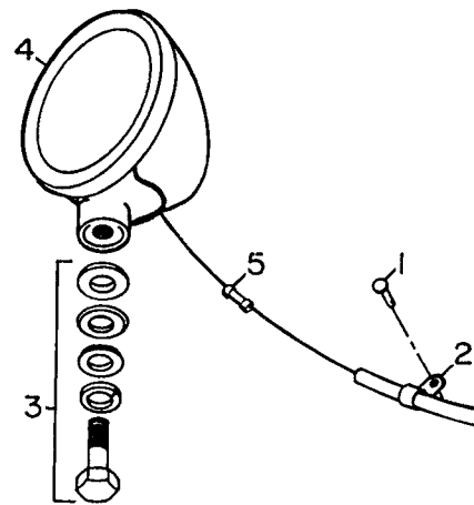
FLOODLIGHT KIT - 12 VOLT - 6 1/2" DIAMETER PART NUMBER 51707613
