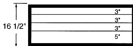
4 - DRAWER 51707862
