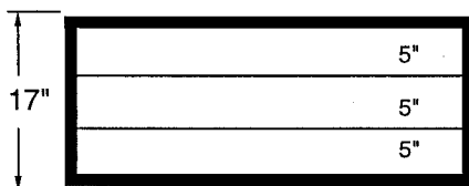
3 - DRAWER 51707861
