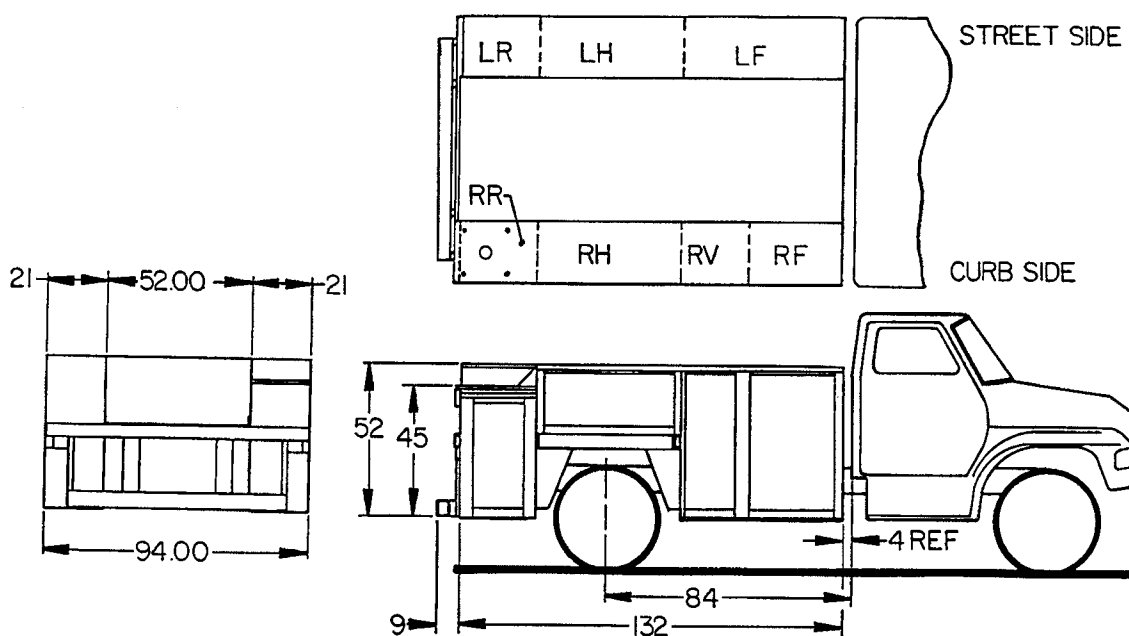
Model 11M940 Mechanics Body REFERENCE DIMENSIONS
