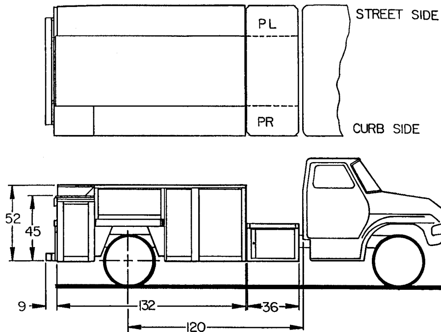
Model 11M940 Mechanics Body with 36" Welder Platform REFERENCE DIMENSIONS
