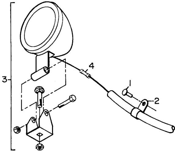
FLOODLIGHT KIT - 12 VOLT - 5" DIAMETER PART NUMBER 51706357
