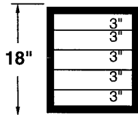
5-DRAWER 51707864
