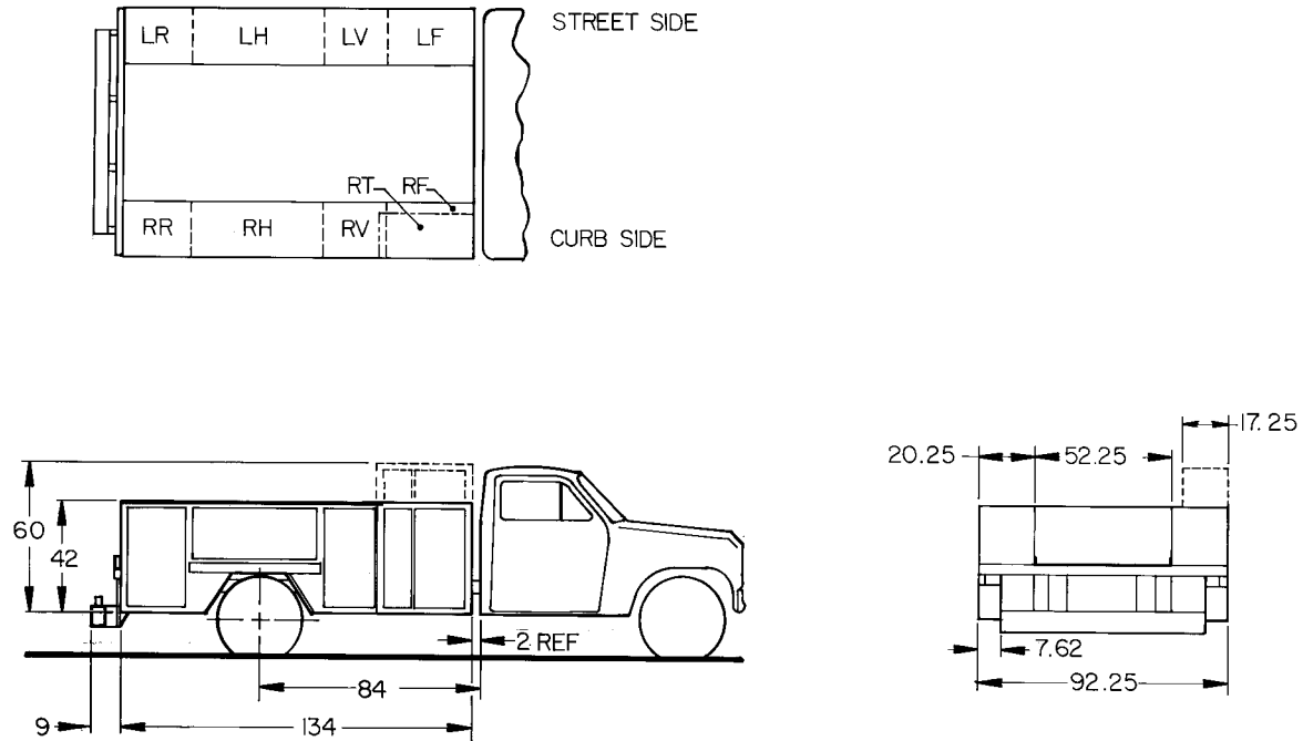
Model 11M920 Mechanics Body REFERENCE DIMENSIONS
