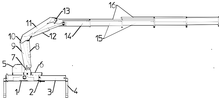
COMPONENT REFERENCE
