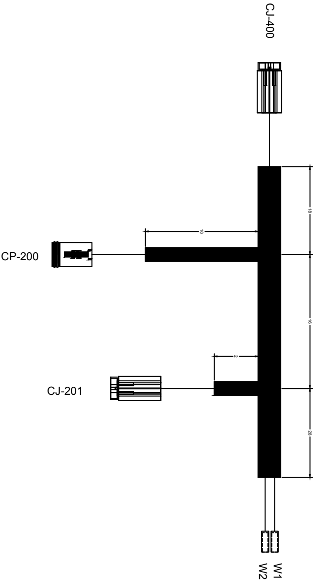
Wiring Harness
